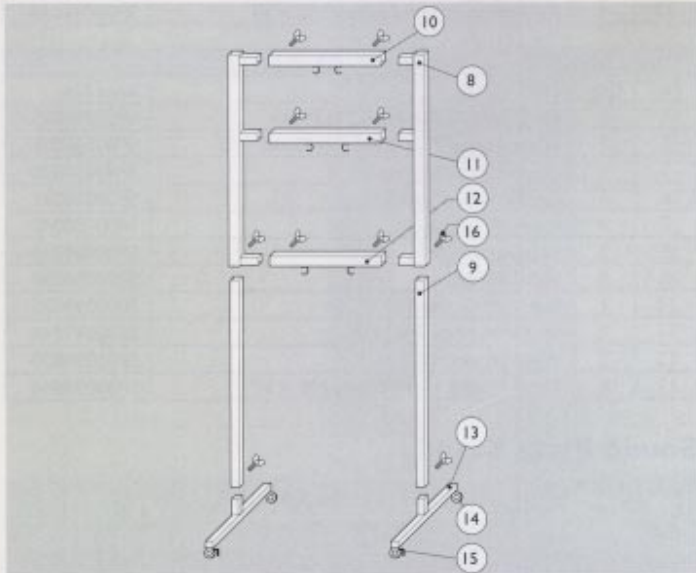
Set Stands No. III for SCG No. 8, 9, 10
